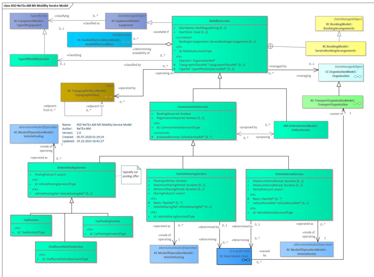
Figure 4: MobilityService (NeTex).
